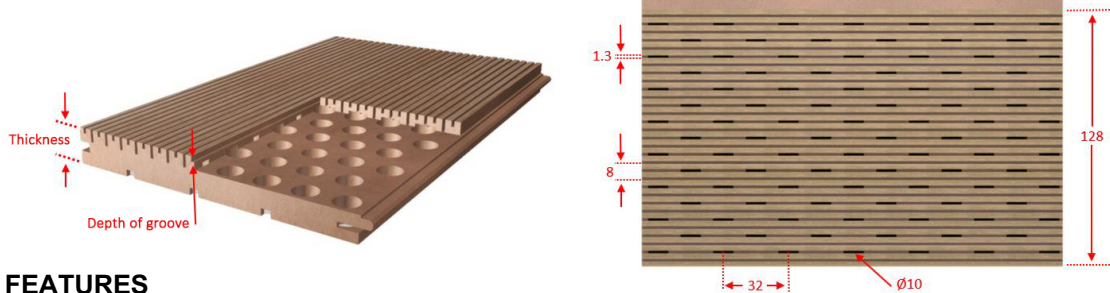
Absorption according UNE-EN ISO 354
